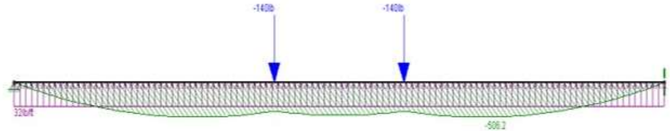
RISA 2-Paddler Moment Diagram
