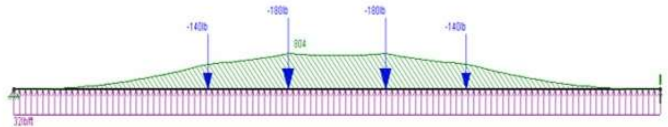
RISA 4-Paddler Moment Diagram
